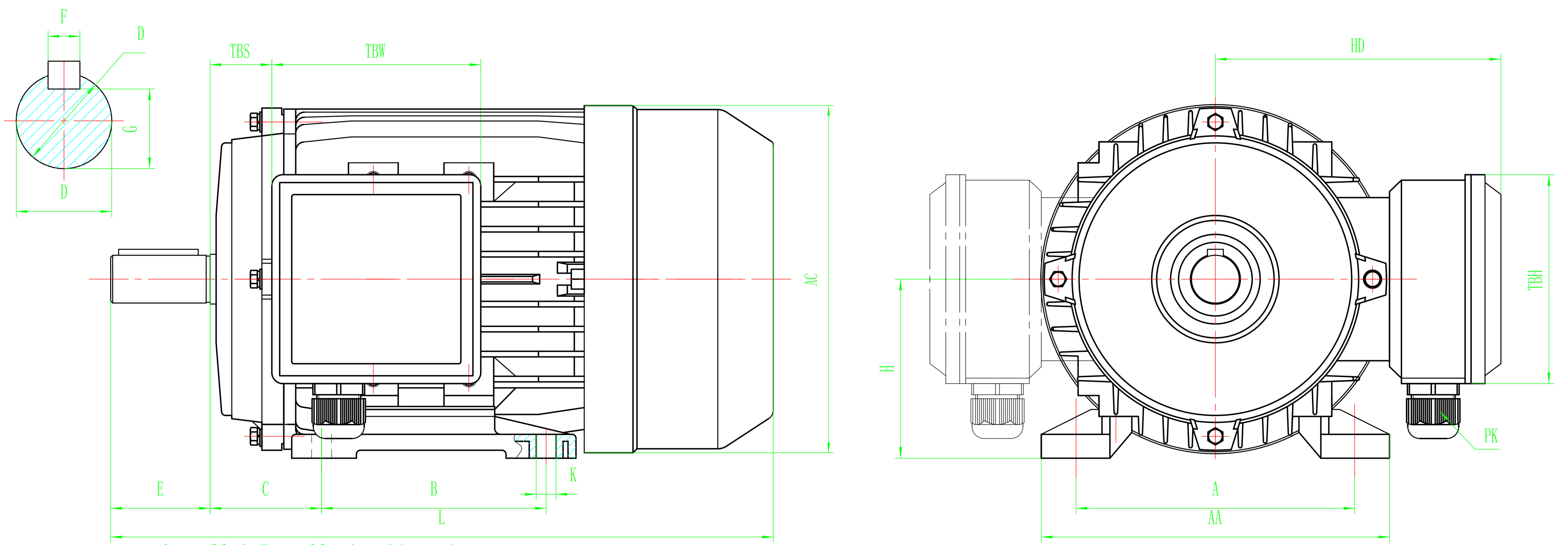
MS56-160 B3 Overall & Installation Dimension
